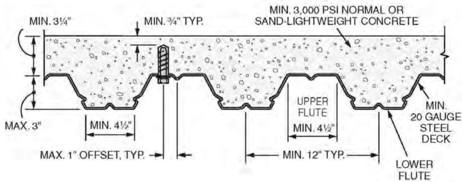
FIGURE 4—INSTALLATION OF 3/8-INCH AND 1/2-INCH SHANK DIAMETER ANCHORS IN THE SOFFIT OF CONCRETE-FILLED PROFILE STEEL DECK FLOOR AND ROOF ASSEMBLIES (UPPER FLUTE) (1 in = 25.4 mm)
