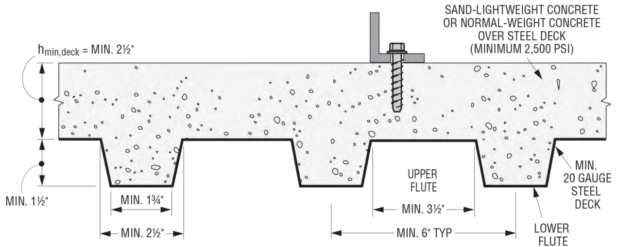
FIGURE 6—INSTALLATION OF 1/4-INCH SHANK DIAMETER ANCHORS IN THE TOPSIDE OF CONCRETE-FILLED PROFILE STEEL DECK FLOOR AND ROOF ASSEMBLIES (1 in = 25.4 mm)
